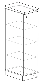
74-40 400x1460x600 74-60 600x1460x600
