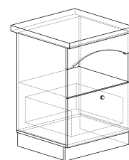
50-60** 600x860x600 50-80** 800x860x600 Hettich
