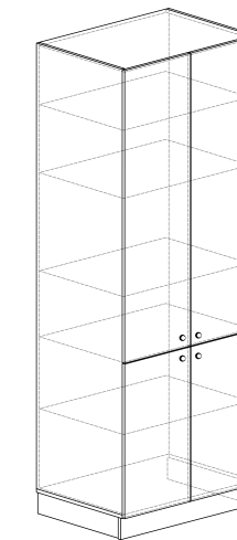
85-80 800x2180x580
