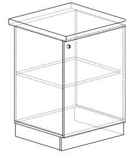
44-15 150x860x600 44-30 300x860x600 44-40 400x860x600 44-45 450x860x600 44-50 500x860x600 44-60 600x860x600
