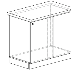
55-100 (лев.) 1000x860x600 55-105 (лев.) 1050x860x600 55-120 (лев.) 1200x860x600
