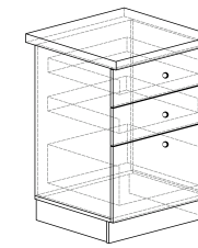
65-40 400x860x600 65-45 450x860x600 65-60 600x860x600 Hettich
